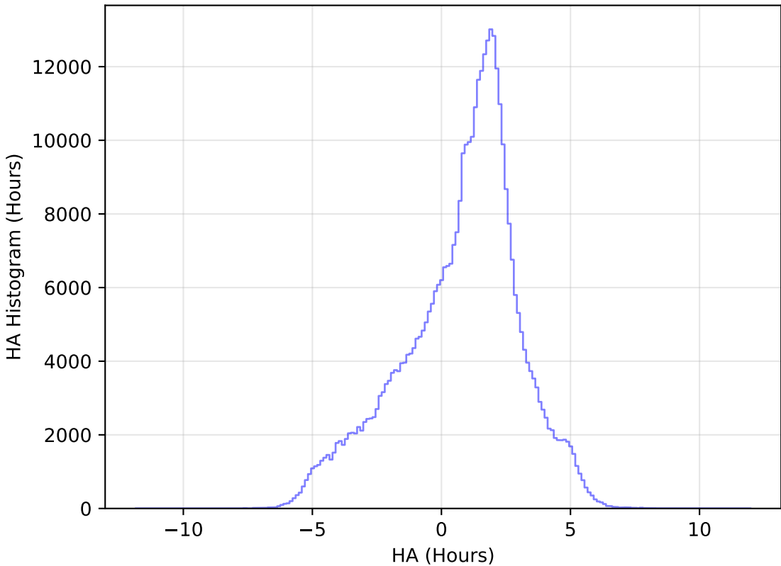
internal_u_expt60_nscale0.9v3.4_10yrs WFD z band: HA Histogram
