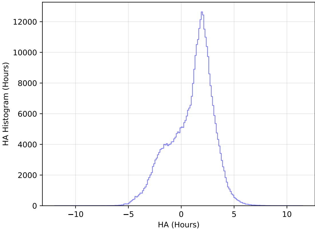
internal_u_expt60_nscale0.9v3.4_10yrs WFD y band: HA Histogram
