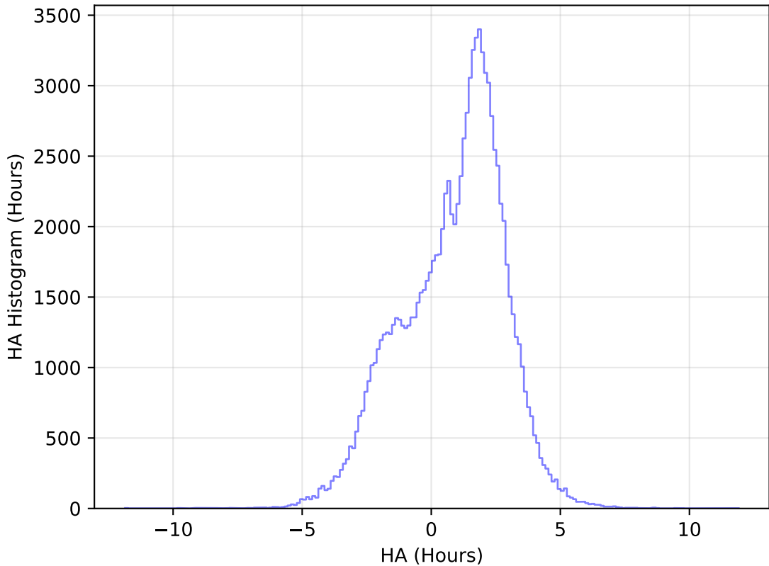
internal_u_expt60_nscale0.9v3.4_10yrs WFD u band: HA Histogram
