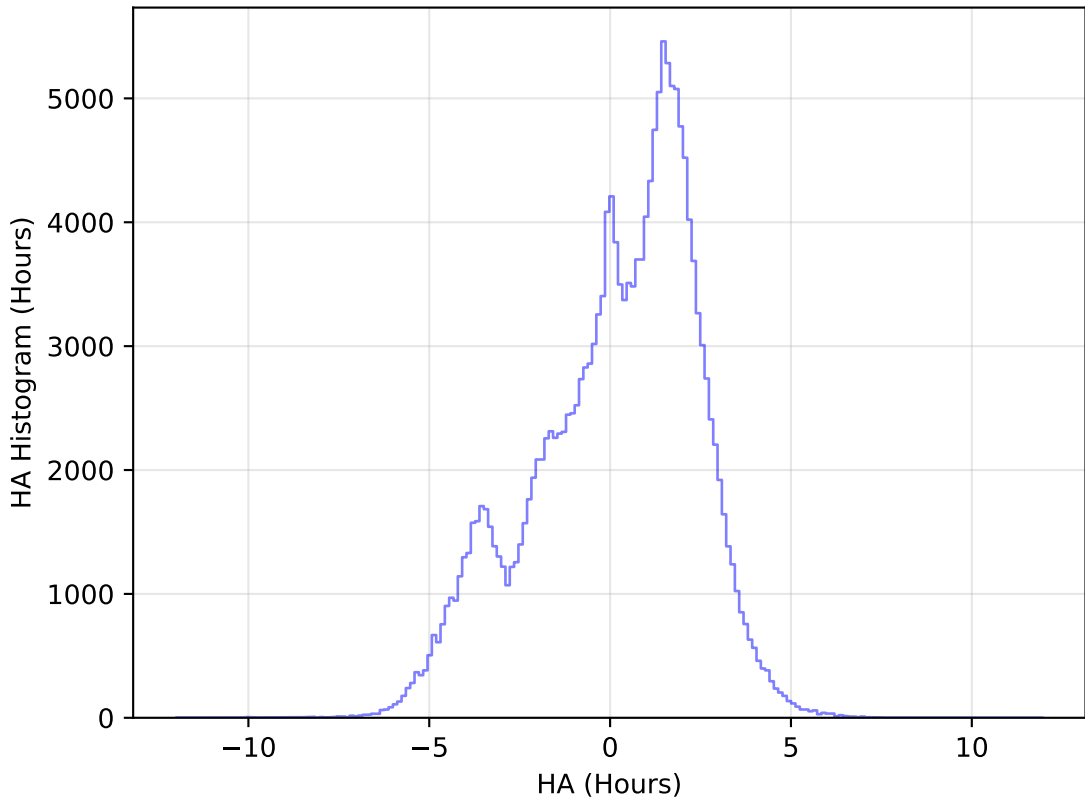
internal_u_expt60_nscale0.9v3.4_10yrs WFD g band: HA Histogram
