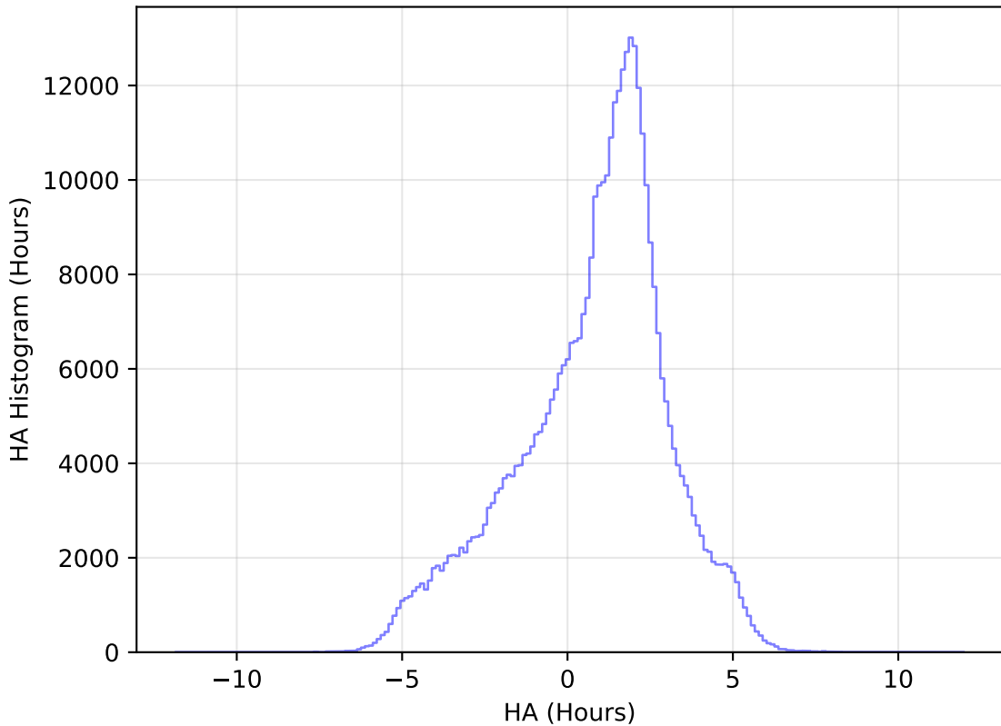
internal_u_expt60_nscale0.9v3.4_10yrs All sky z band: HA Histogram
