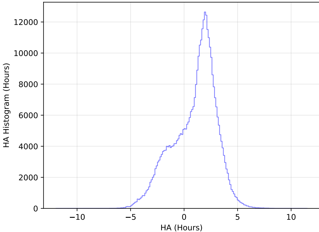
internal_u_expt60_nscale0.9v3.4_10yrs All sky y band: HA Histogram
