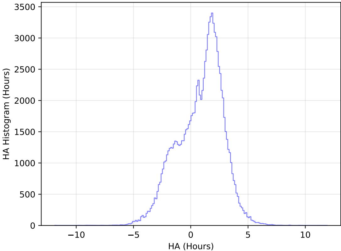
internal_u_expt60_nscale0.9v3.4_10yrs All sky u band: HA Histogram
