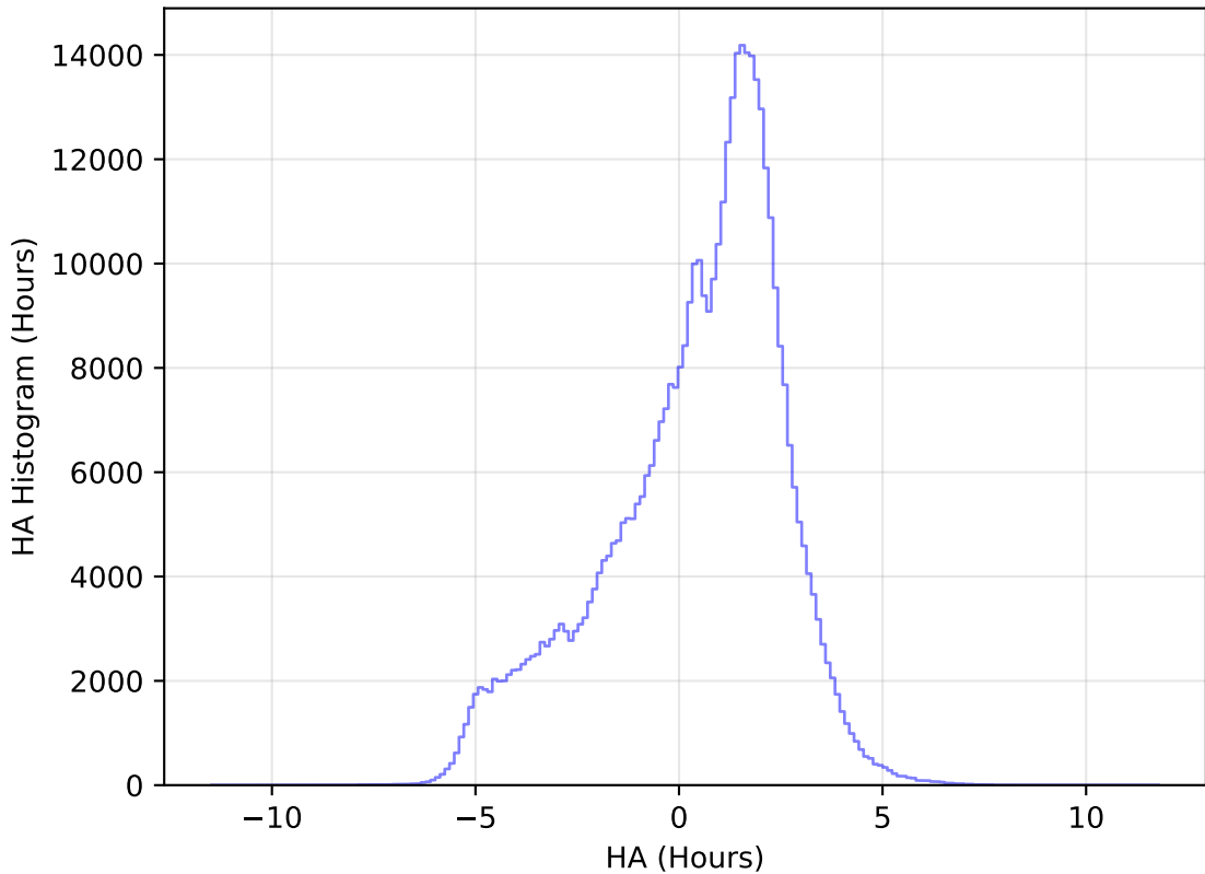
internal_u_expt60_nscale0.9v3.4_10yrs All sky r band: HA Histogram
