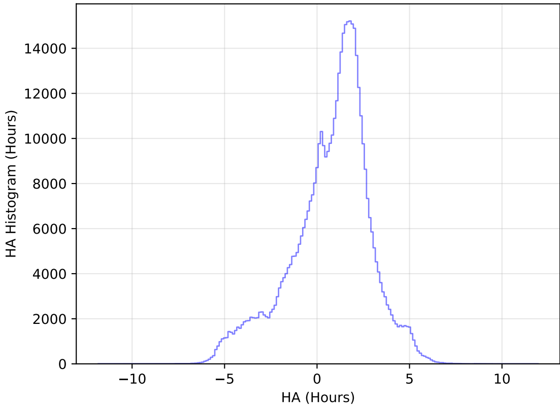
internal_u_expt60_nscale0.9v3.4_10yrs All sky i band: HA Histogram
