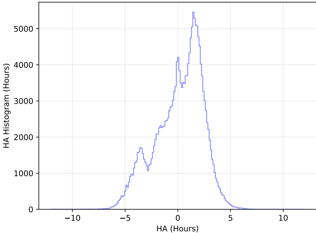
internal_u_expt60_nscale0.9v3.4_10yrs All sky g band: HA Histogram
