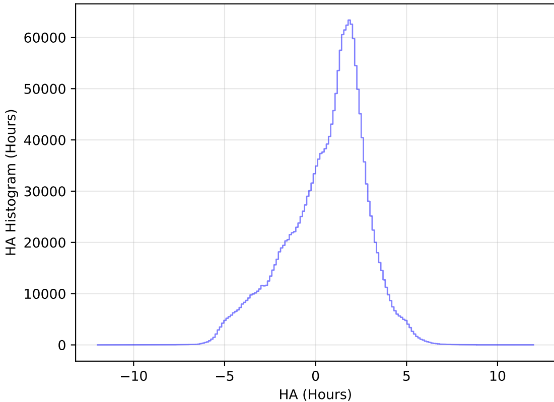
internal_u_expt60_nscale0.9v3.4_10yrs All sky all bands: HA Histogram
