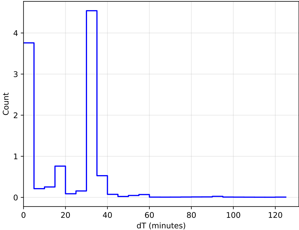
internal_u_expt60_nscale0.9v3.4_10yrs WFD: DeltaT Histogram
