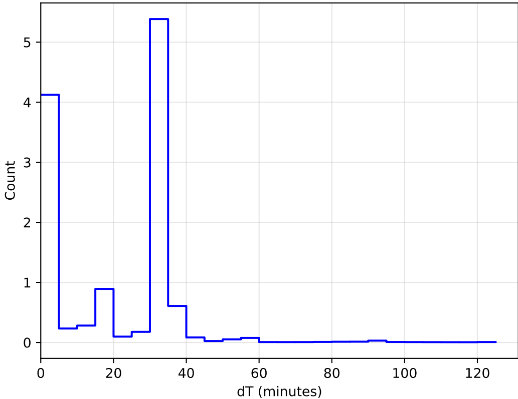
internal_u_expt60_nscale0.9v3.4_10yrs All sky: DeltaT Histogram
