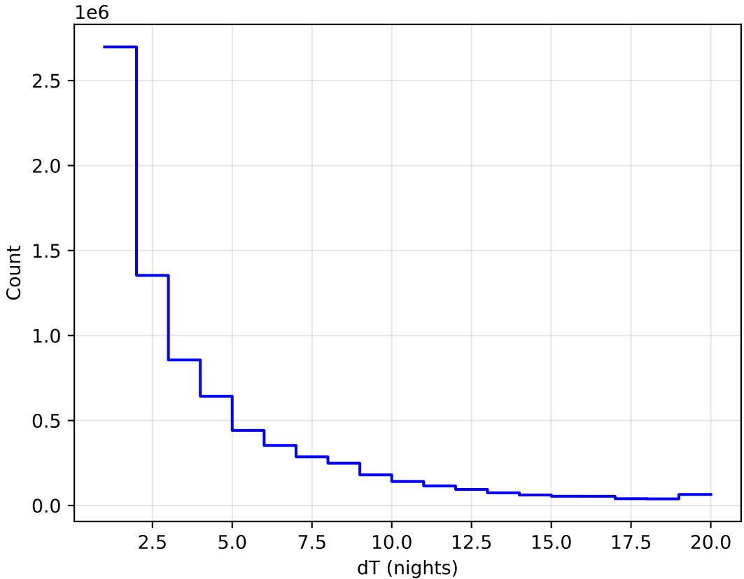
internal_u_expt60_nscale0.9v3.4_10yrs WFD all bands: DeltaNight Histogram
