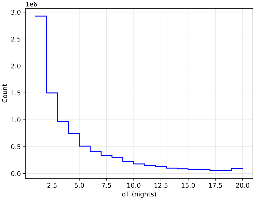
internal_u_expt60_nscale0.9v3.4_10yrs All sky all bands: DeltaNight Histogram
