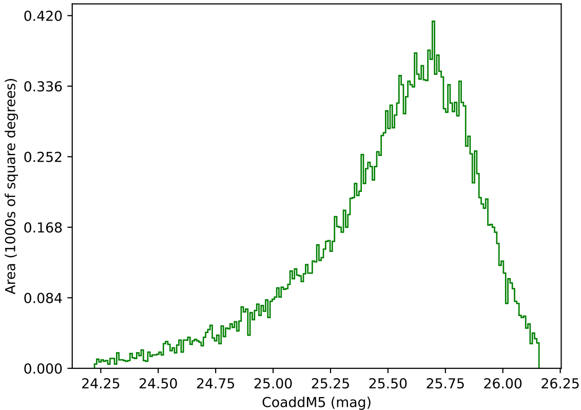
internal_u_expt60_nscale0.9v3.4_10yrs Yr 1 g band: CoaddM5
