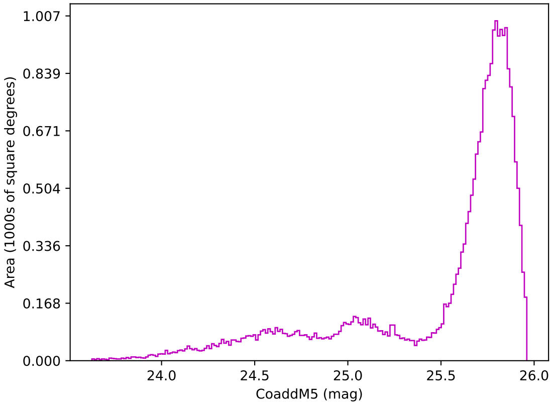
internal_u_expt60_nscale0.9v3.4_10yrs All sky z band: CoaddM5
