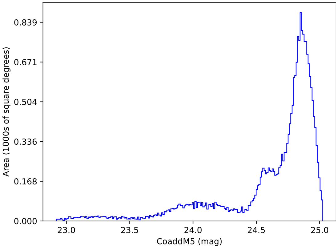
internal_u_expt60_nscale0.9v3.4_10yrs All sky y band: CoaddM5
