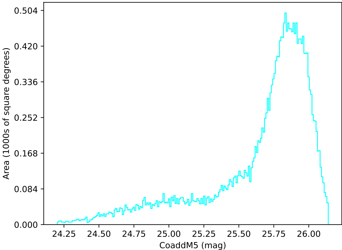
internal_u_expt60_nscale0.9v3.4_10yrs All sky u band: CoaddM5
