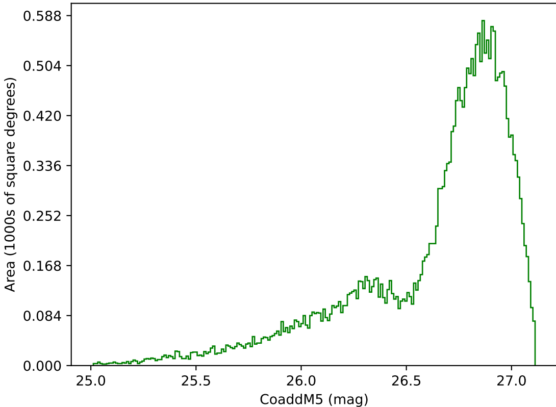
internal_u_expt60_nscale0.9v3.4_10yrs All sky g band: CoaddM5
