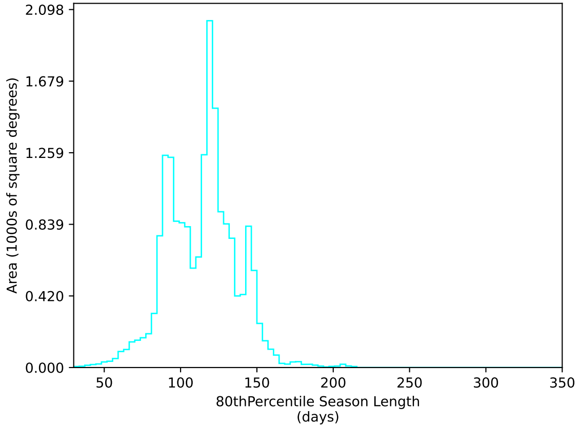
internal_u_expt60_nscale0.9v3.4_10yrs WFD u band: 80thPercentile Season Length
