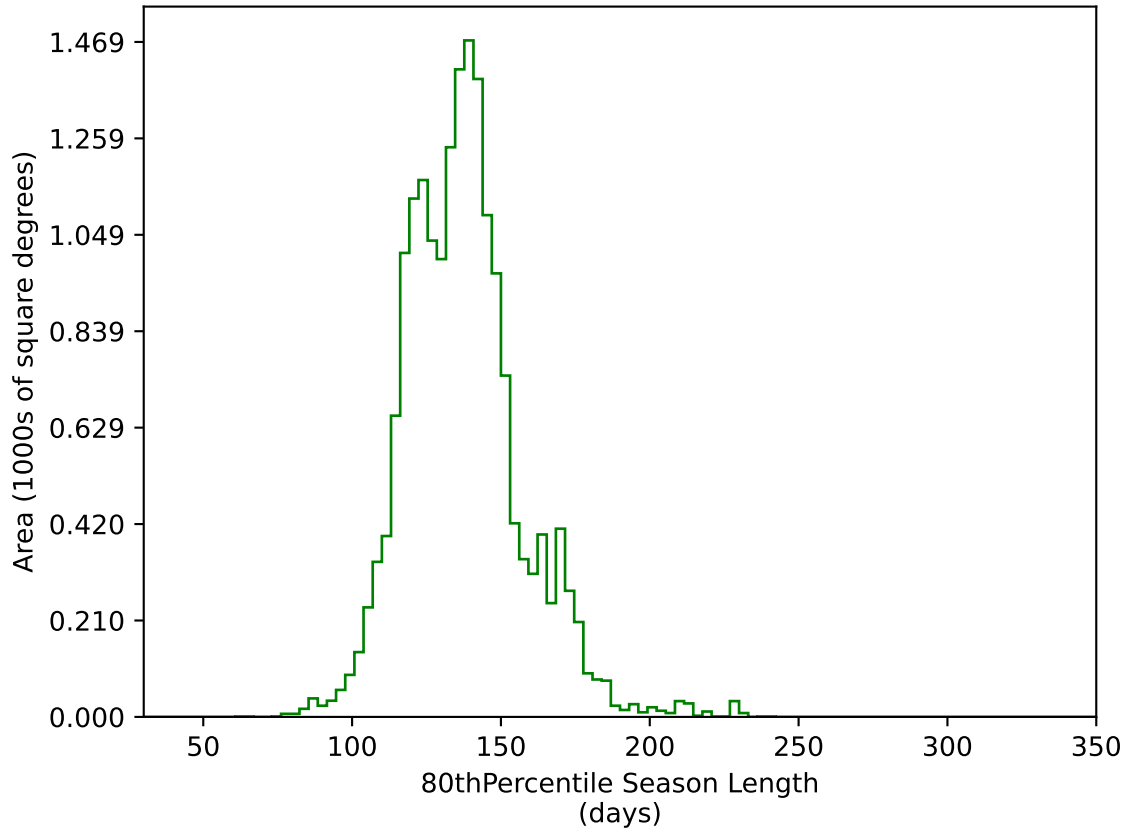
internal_u_expt60_nscale0.9v3.4_10yrs WFD g band: 80thPercentile Season Length
