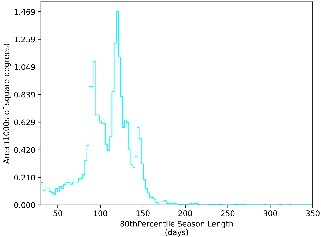
internal_u_expt60_nscale0.9v3.4_10yrs All sky u band: 80thPercentile Season Length
