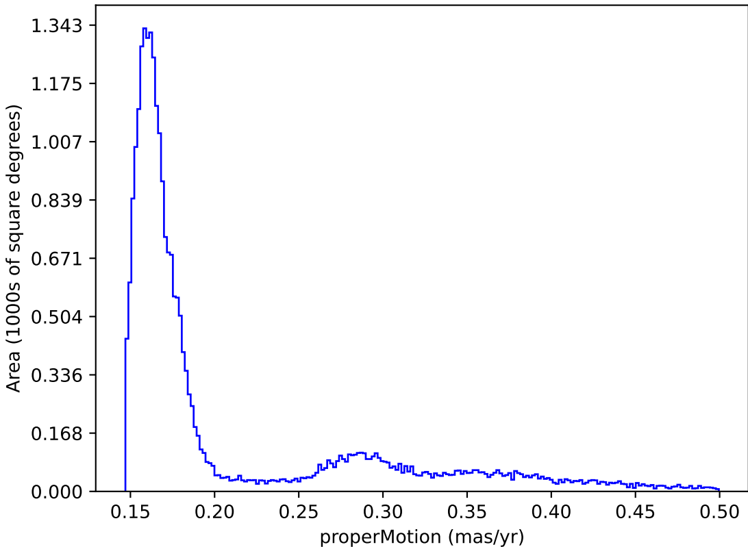
internal_u_expt60_nscale0.9v3.4_10yrs : properMotion
