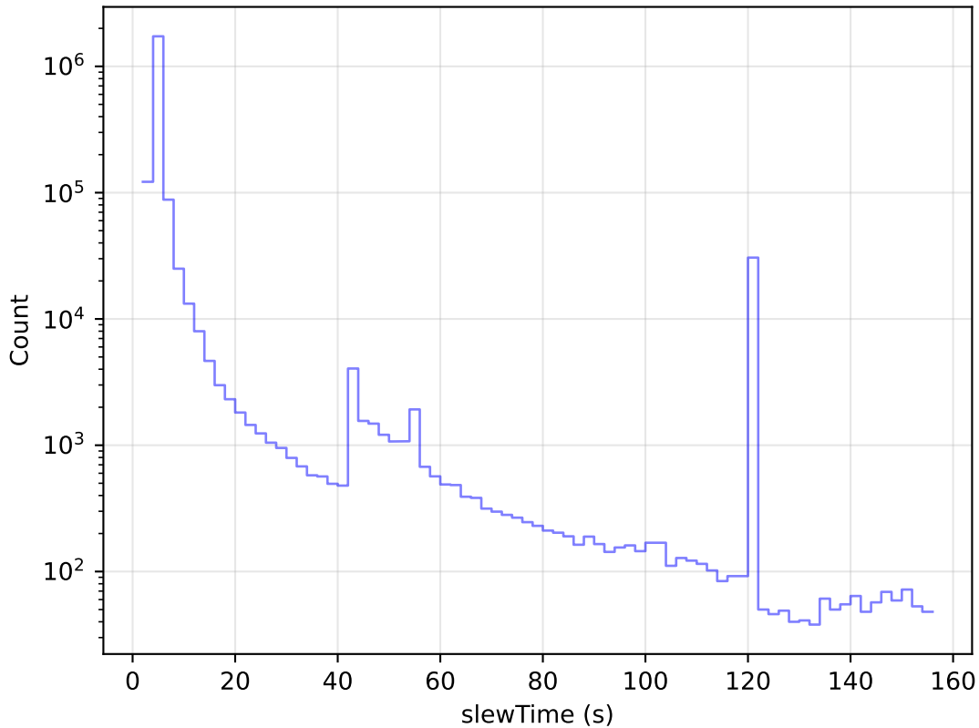
internal_u_expt60_nscale0.9v3.4_10yrs All visits: Slew Time Histogram
