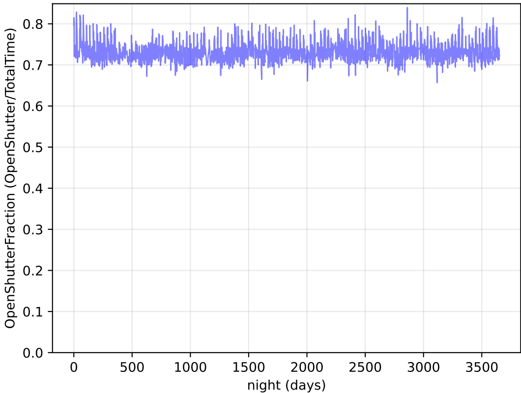
internal_u_expt60_nscale0.9v3.4_10yrs : OpenShutterFraction
