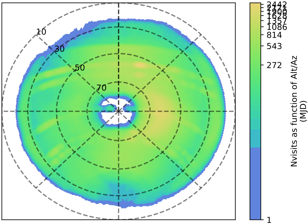
internal_u_expt60_nscale0.9v3.4_10yrs z: Nvisits as function of Alt/Az
