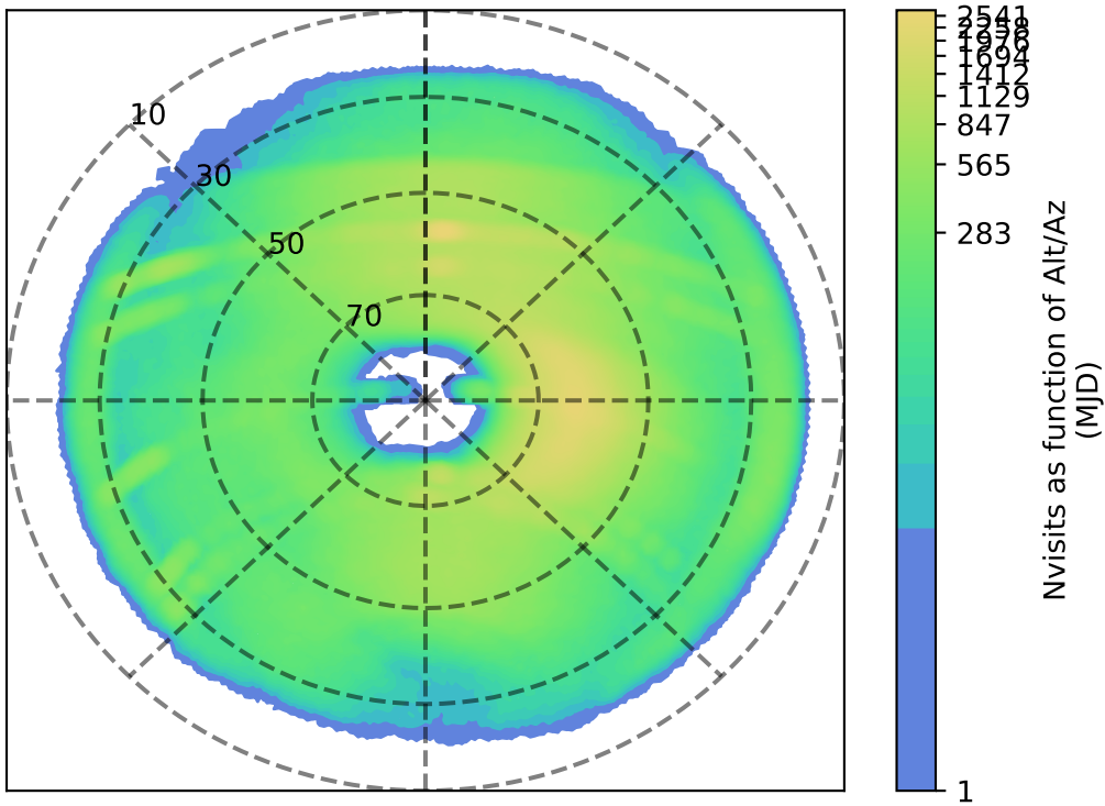
internal_u_expt60_nscale0.9v3.4_10yrs i: Nvisits as function of Alt/Az
