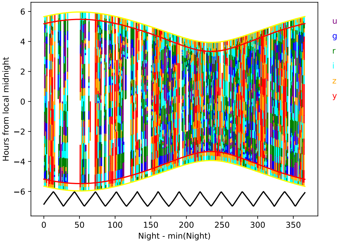
internal_u_expt60_nscale0.9v3.4_10yrs year 8-9: Hourglass
