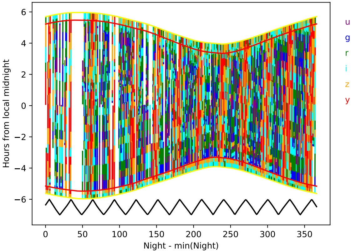
internal_u_expt60_nscale0.9v3.4_10yrs year 6-7: Hourglass
