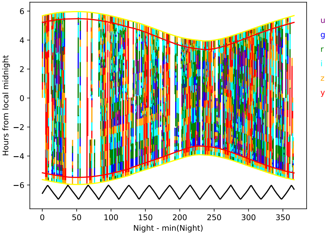
internal_u_expt60_nscale0.9v3.4_10yrs year 3-4: Hourglass
