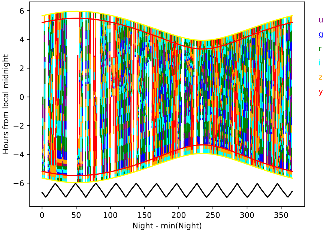
internal_u_expt60_nscale0.9v3.4_10yrs year 2-3: Hourglass
