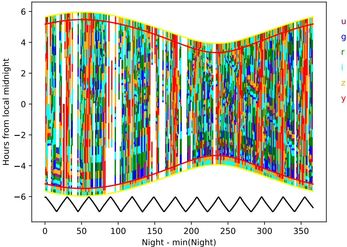
internal_u_expt60_nscale0.9v3.4_10yrs year 1-2: Hourglass
