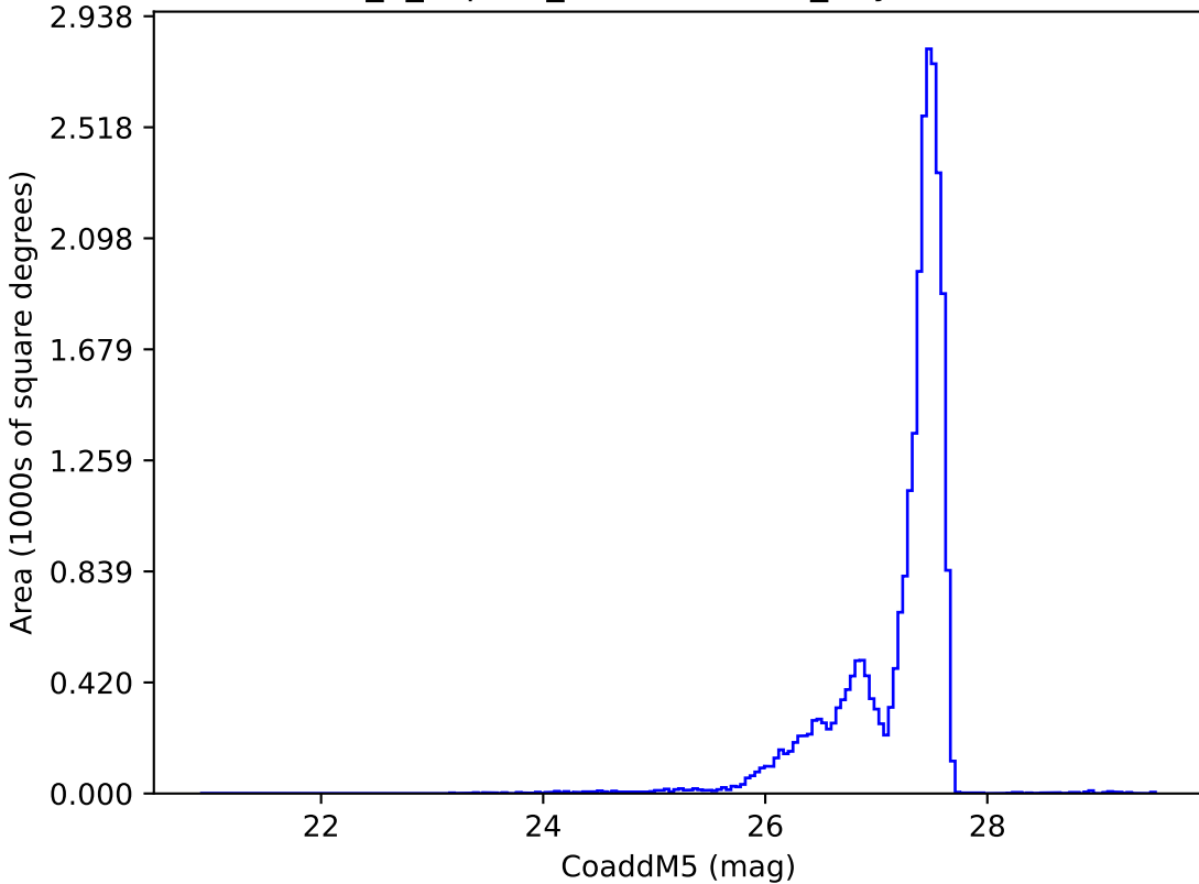
internal_u_expt60_nscale0.9v3.4_10yrs : CoaddM5
