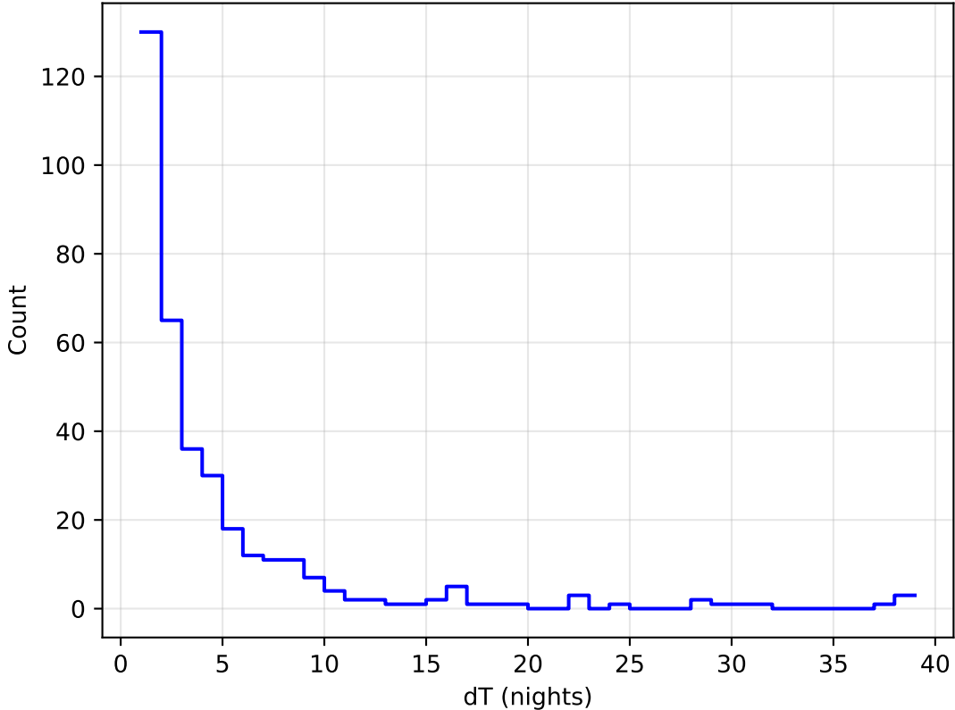
internal_u_expt60_nscale0.9v3.4_10yrs all bands: DD:WFD Delta Nights Histogram
