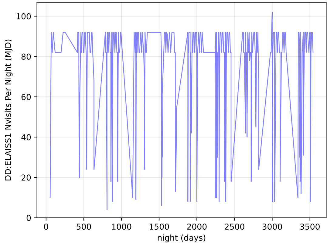
internal_u_expt60_nscale0.9v3.4_10yrs all bands: DD:ELAISS1 Nvisits Per Night
