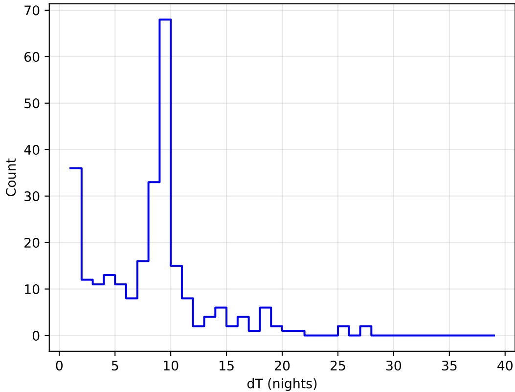
internal_u_expt60_nscale0.9v3.4_10yrs all bands: DD:ELAISS1 Delta Nights Histogram
