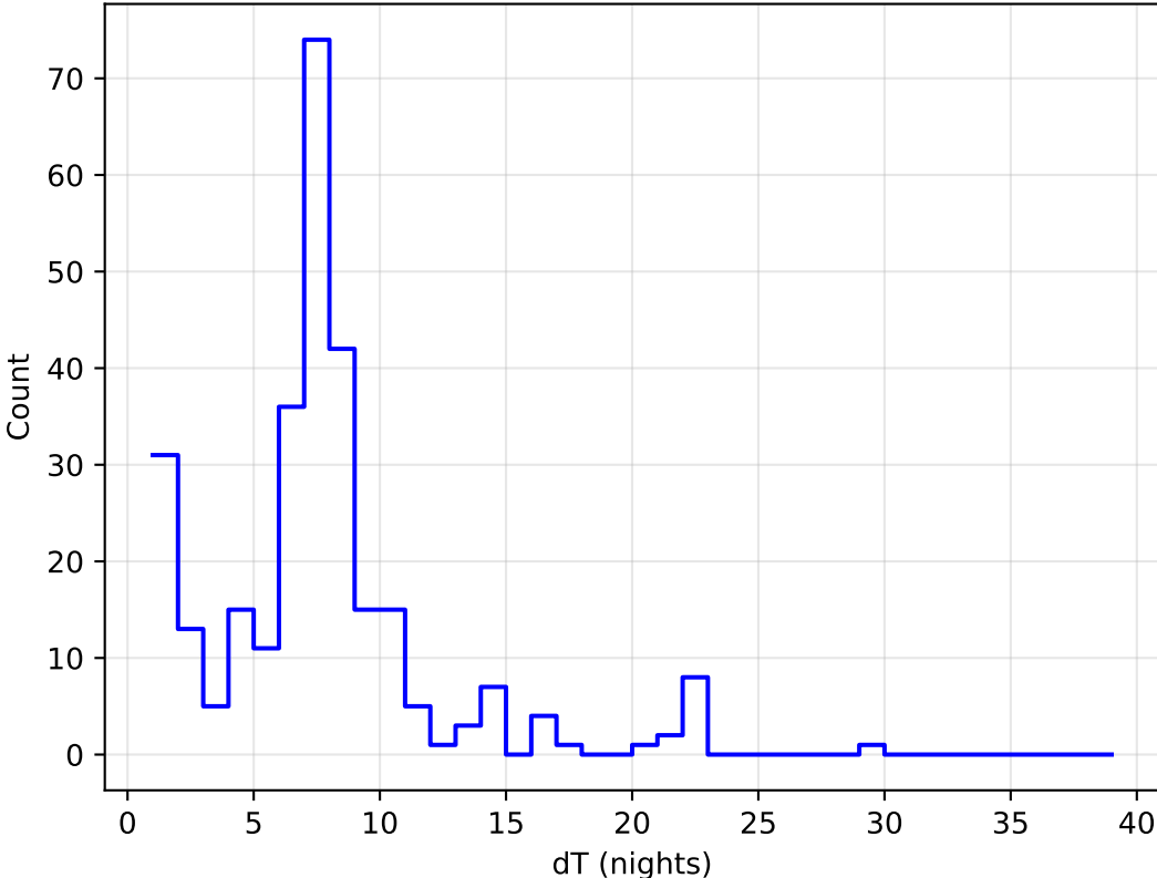
internal_u_expt60_nscale0.9v3.4_10yrs all bands: DD:EDFS Delta Nights Histogram
