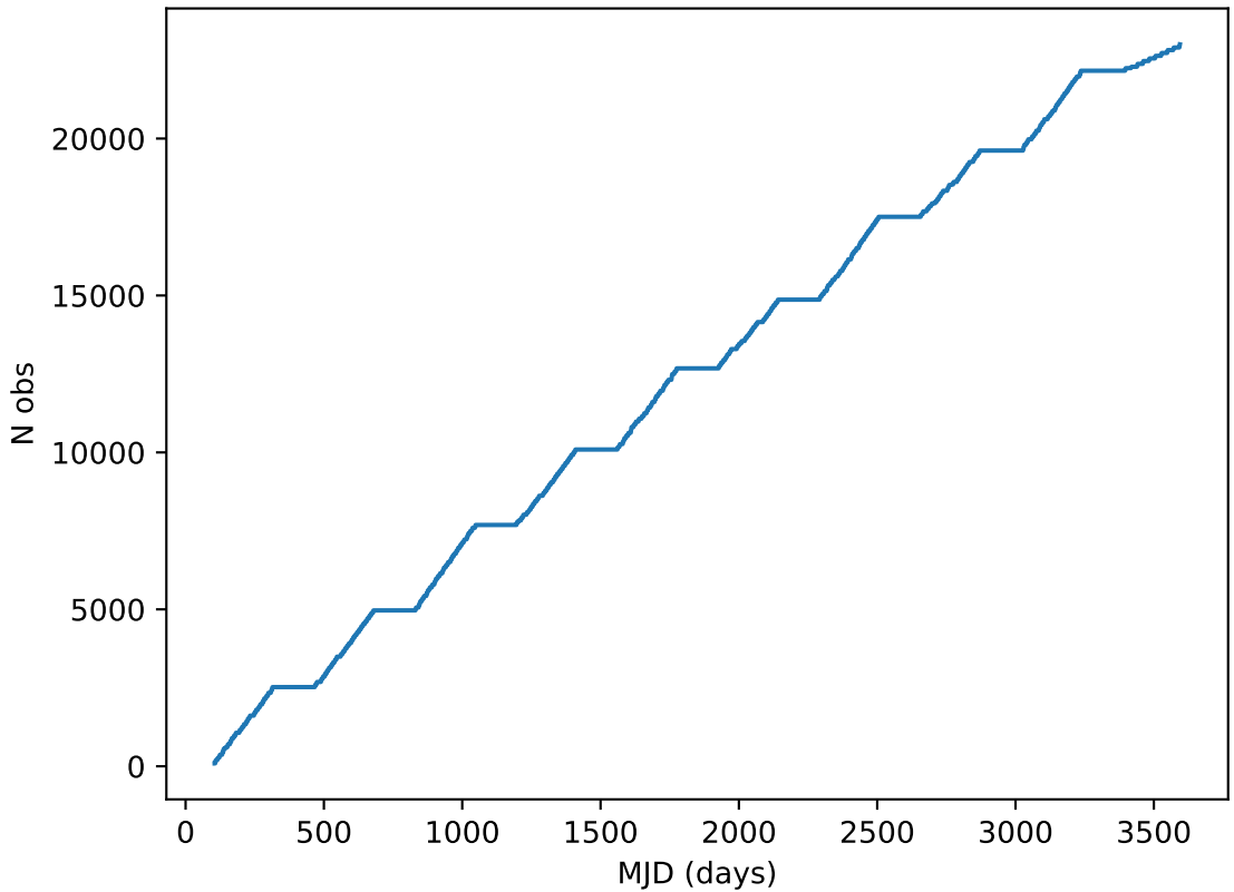
internal_u_expt60_nscale0.9v3.4_10yrs all bands: DD:EDFS Cumulative NVisits
