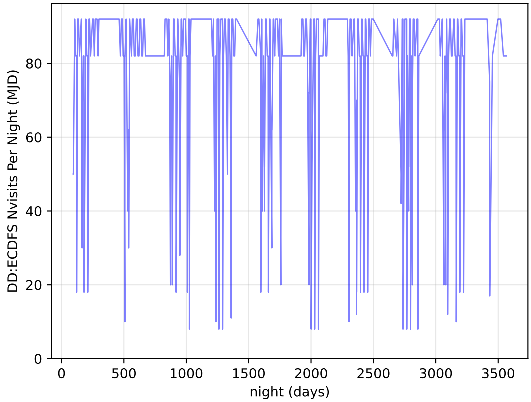
internal_u_expt60_nscale0.9v3.4_10yrs all bands: DD:ECDFS Nvisits Per Night
