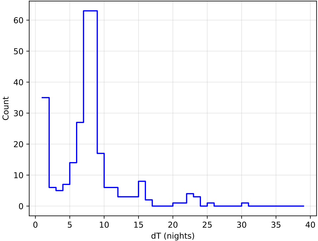
internal_u_expt60_nscale0.9v3.4_10yrs all bands: DD:ECDFS Delta Nights Histogram
