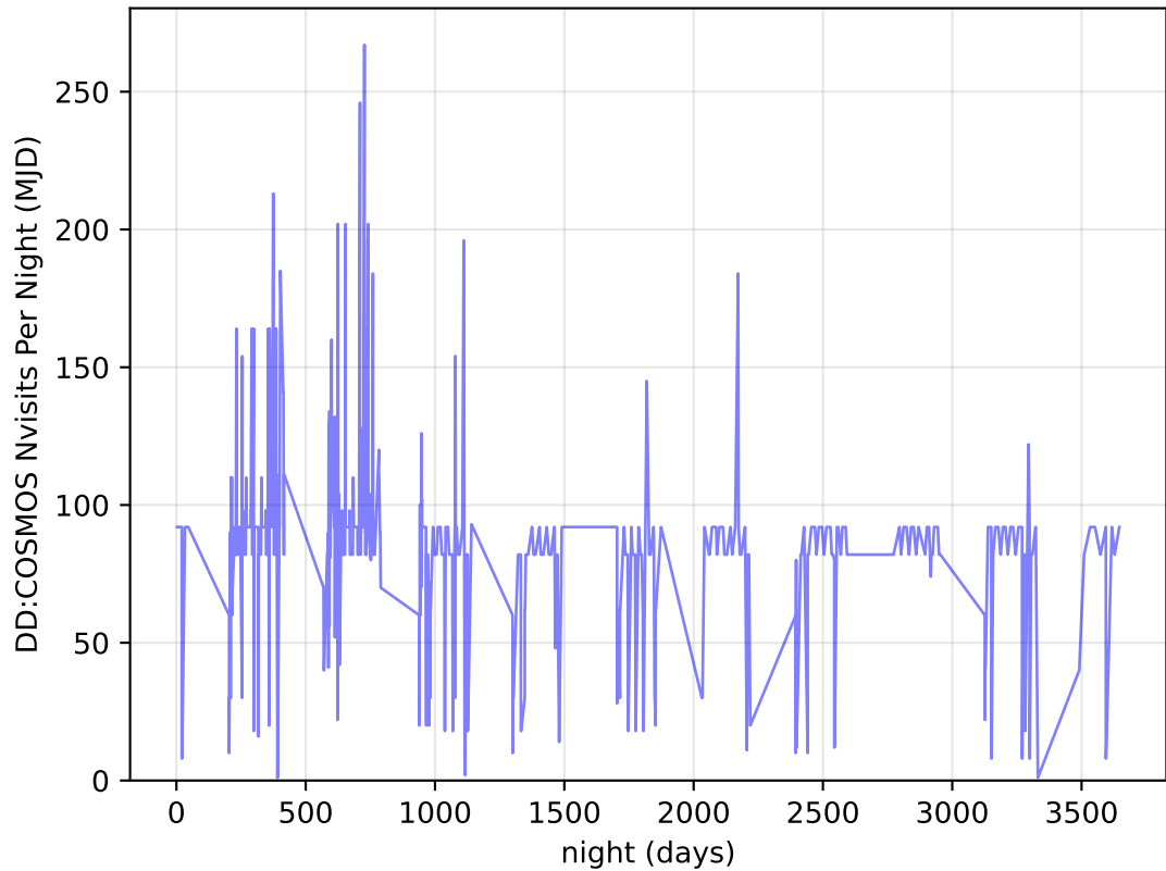
internal_u_expt60_nscale0.9v3.4_10yrs all bands: DD: COSMOS Nvisits Per Night
