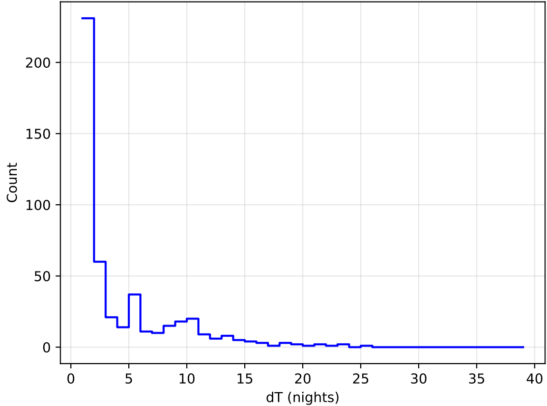
internal_u_expt60_nscale0.9v3.4_10yrs all bands: DD:COSMOS Delta Nights Histogram
