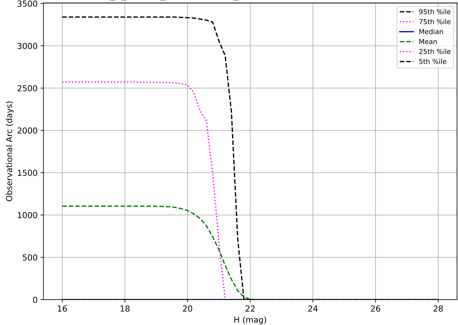
internal_u_expt45_nscale1.5v3.4_10yrs: Observational Arc Length Vatira
