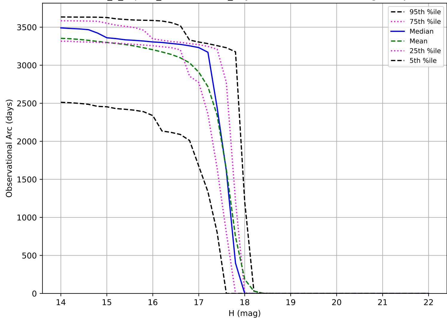
internal_u_expt45_nscale1.5v3.4_10yrs: Observational Arc Length Trojan
