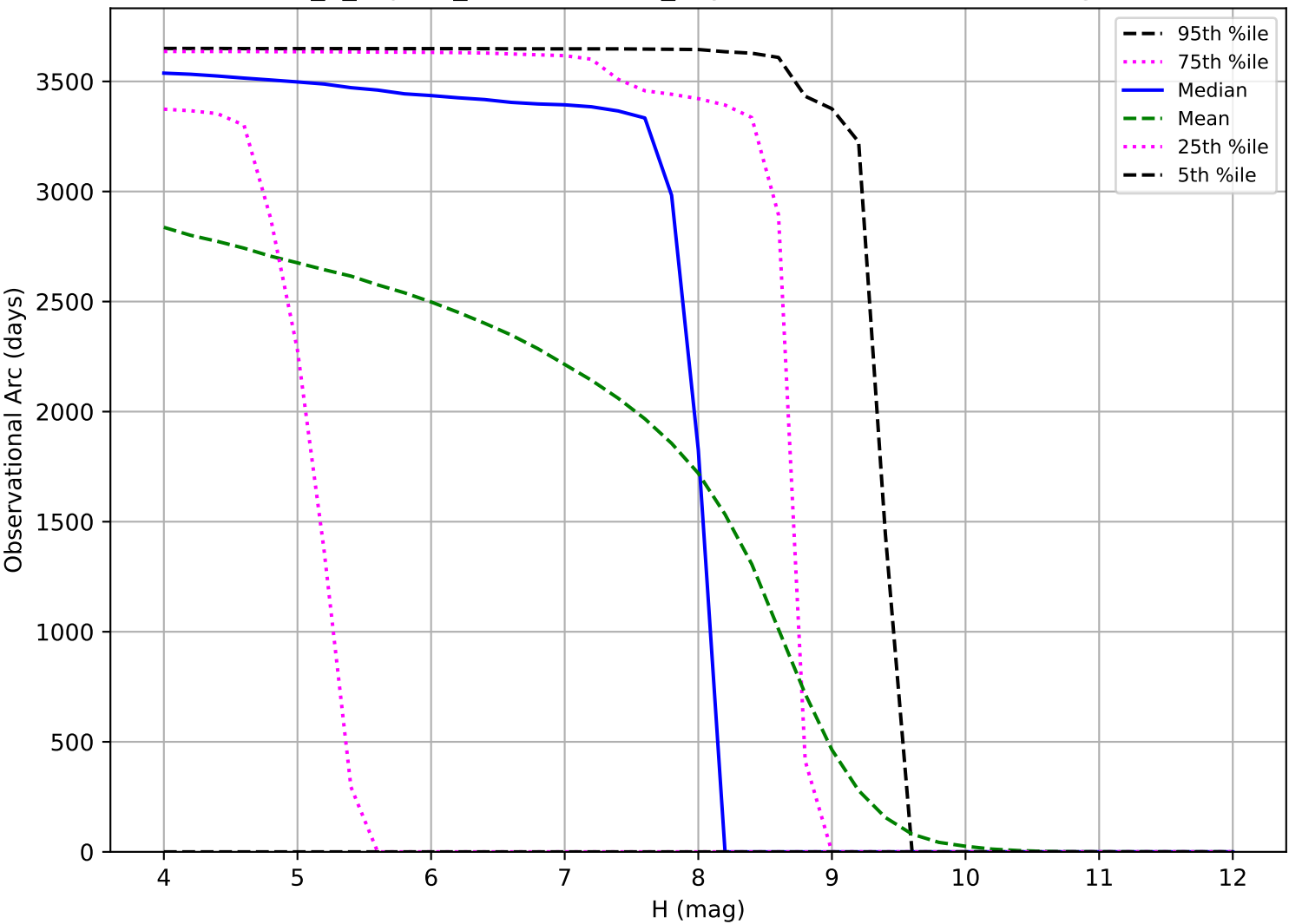
internal_u_expt45_nscale1.5v3.4_10yrs: Observational Arc Length TNO
