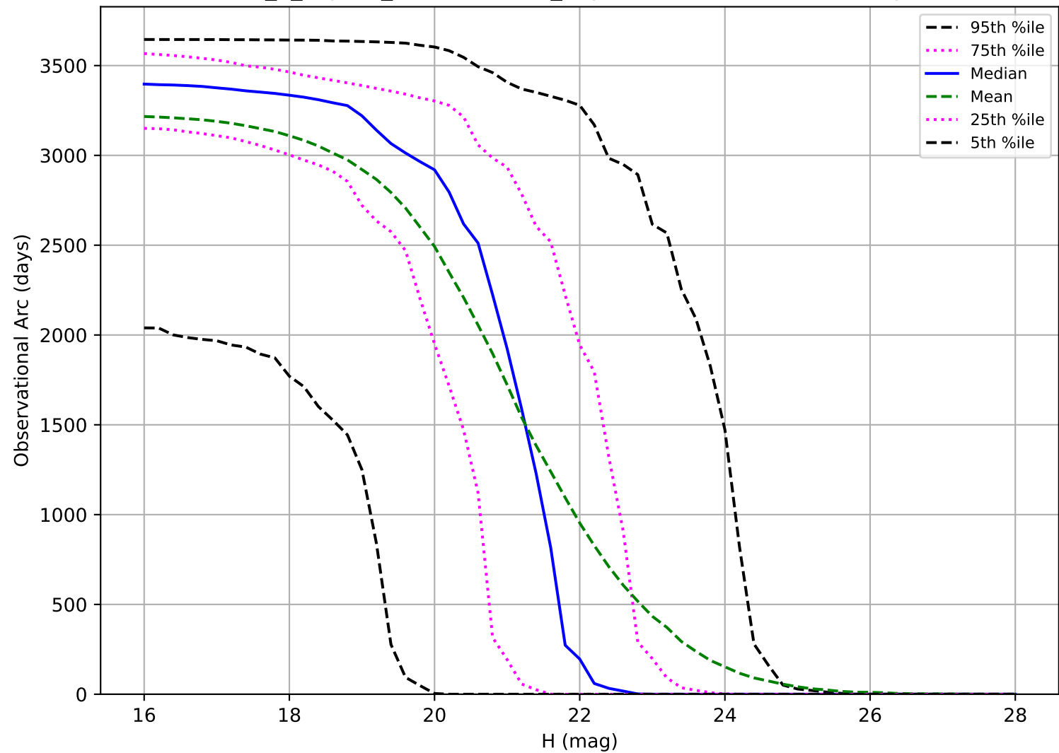
internal_u_expt45_nscale1.5v3.4_10yrs: Observational Arc Length PHA
