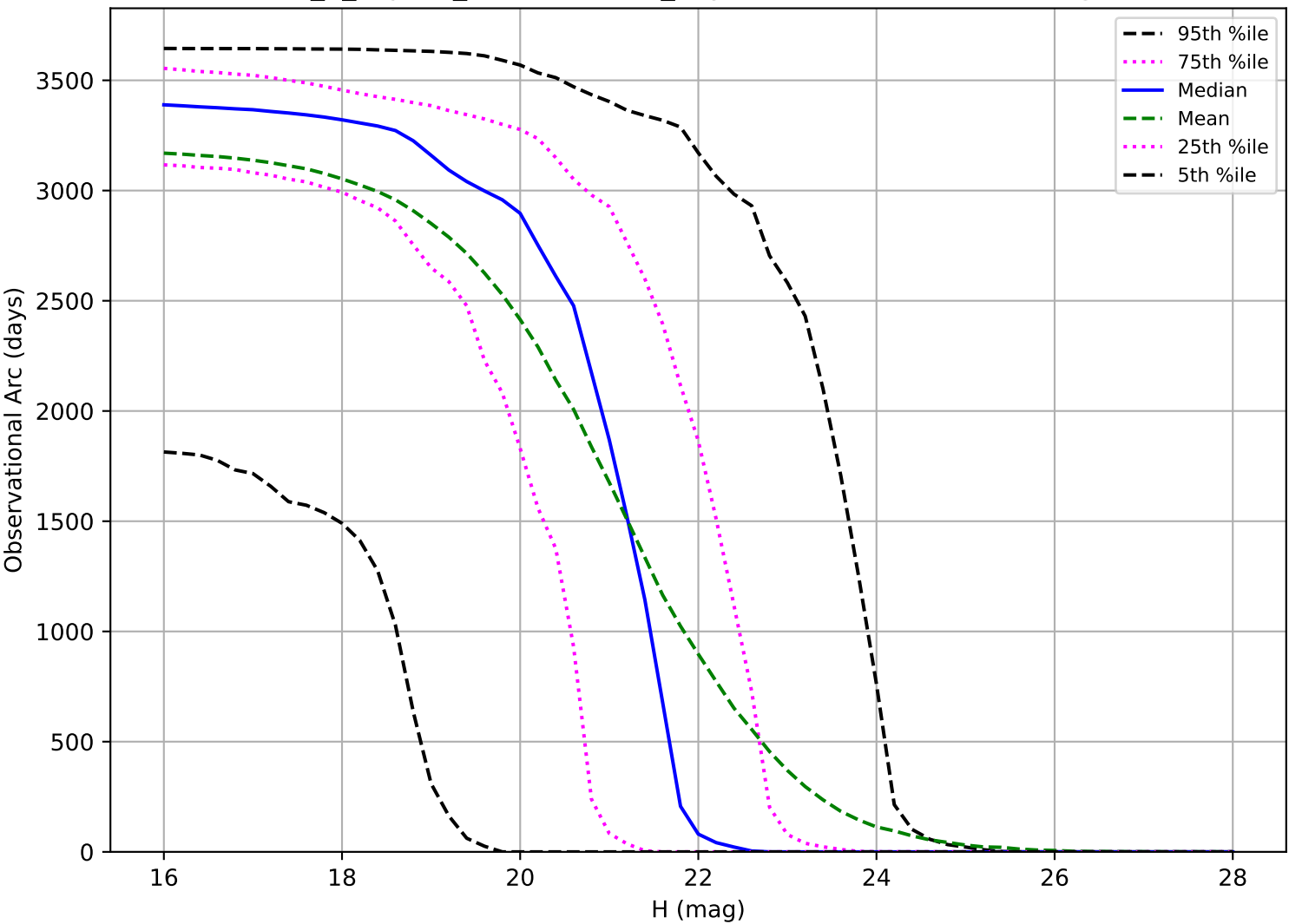
internal_u_expt45_nscale1.5v3.4_10yrs: Observational Arc Length NEO
