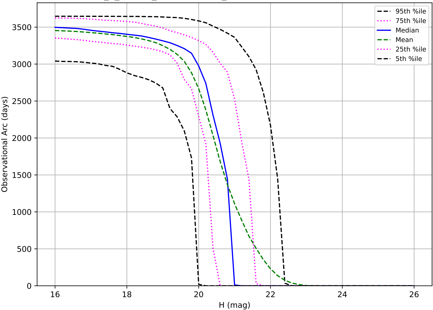
internal_u_expt45_nscale1.5v3.4_10yrs: Observational Arc Length MBA
