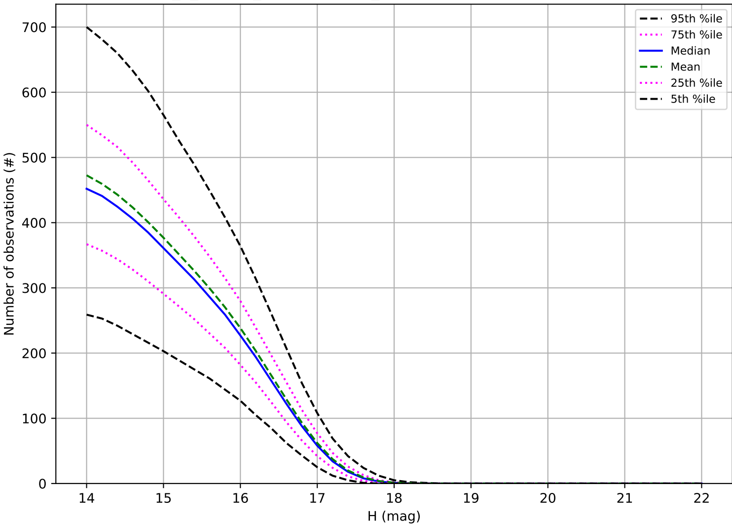
internal_u_expt45_nscale1.5v3.4_10yrs: Number of observations Trojan
